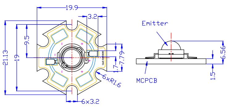
Unit:mm Tolerances are for reference only
